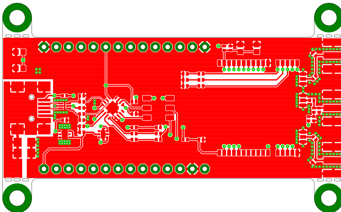
Figure 2: Top copper layer of EVAL TT-SU2
