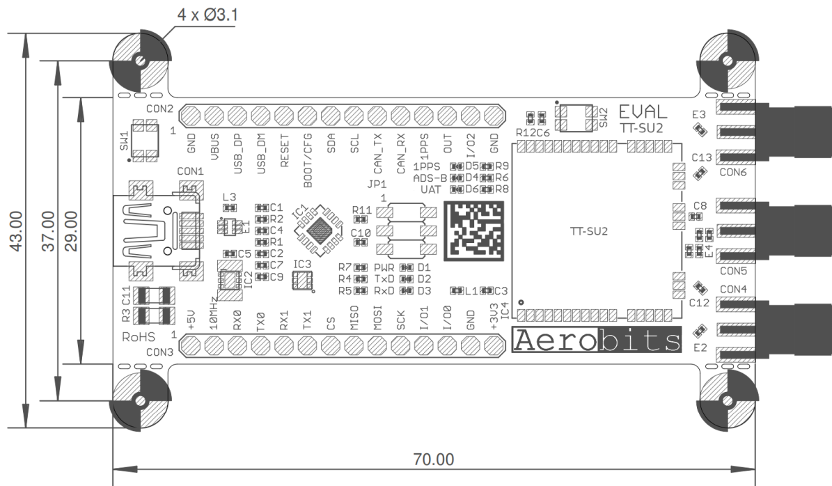
Figure 5: Dimensions of EVAL TT-SU2
