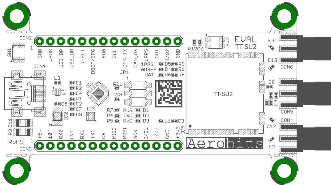
Figure 1: Top view of EVAL TT-SU2.
