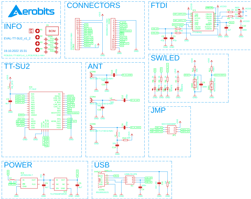
Figure 4: Electrical diagram of EVAL TT-SU2
