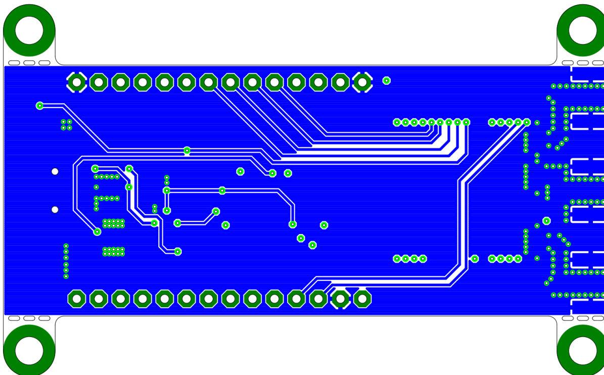
Figure 3: Bottom copper layer of EVAL TT-SU2
