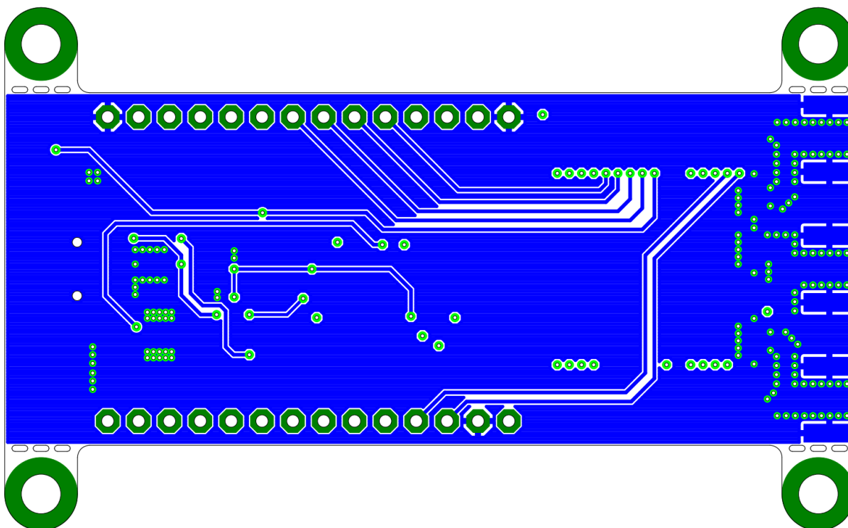
Figure 3: Bottom copper layer of EVAL TT-SG1
