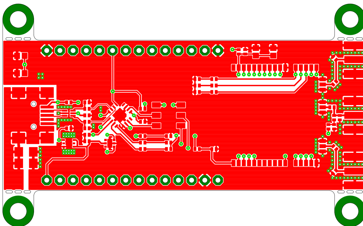
Figure 2: Top copper layer of EVAL TT-SG1
