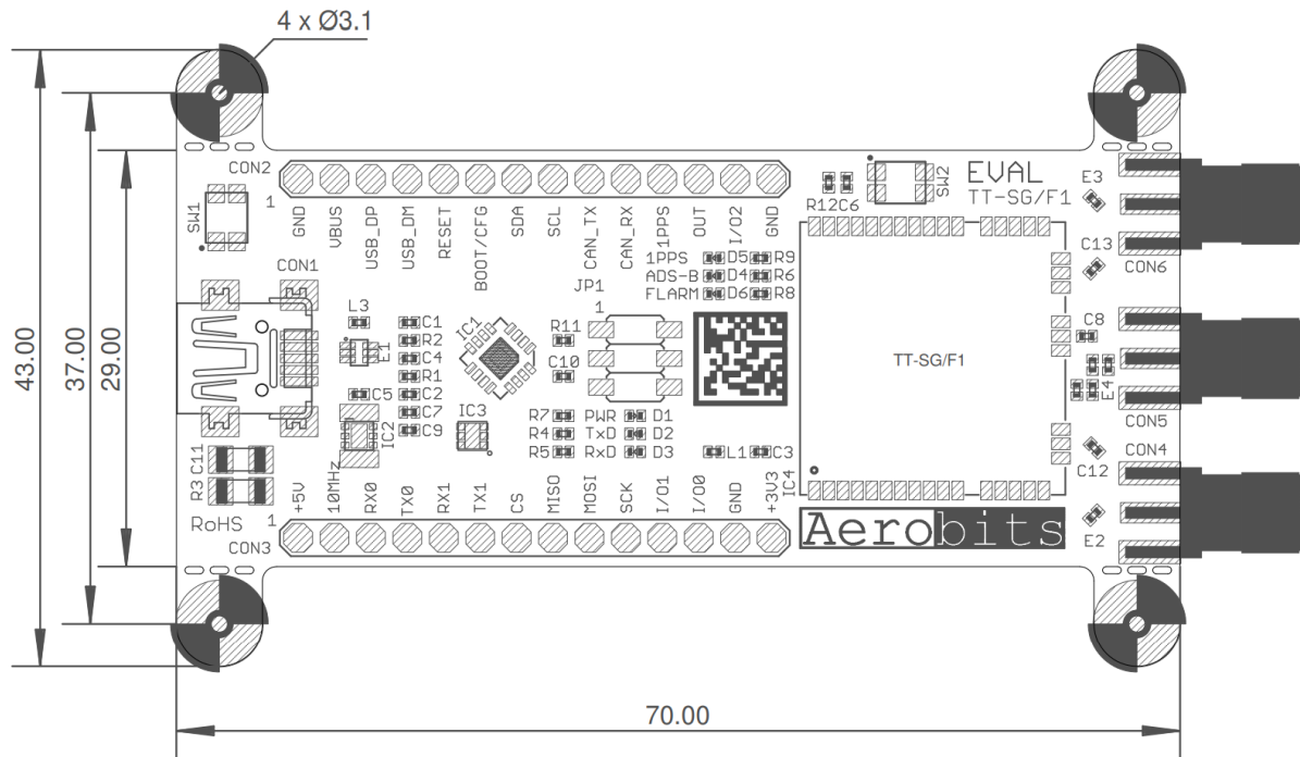
Figure 5: Dimensions of EVAL TT-SG1
