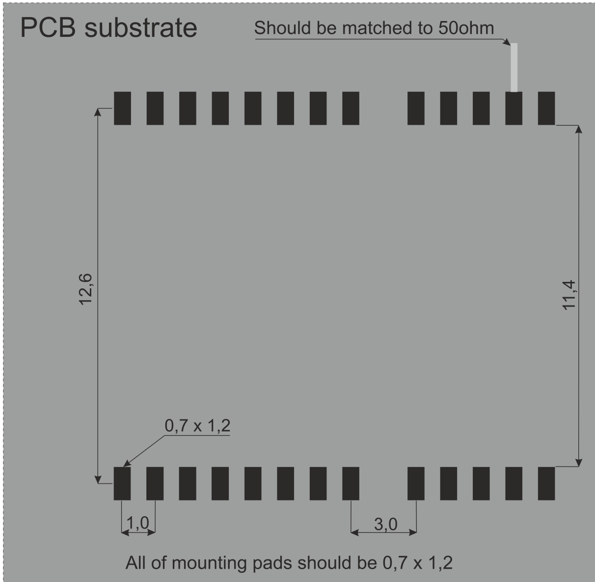
Figure 3: Footprint of OEM TT-SC1 EXTENDED
