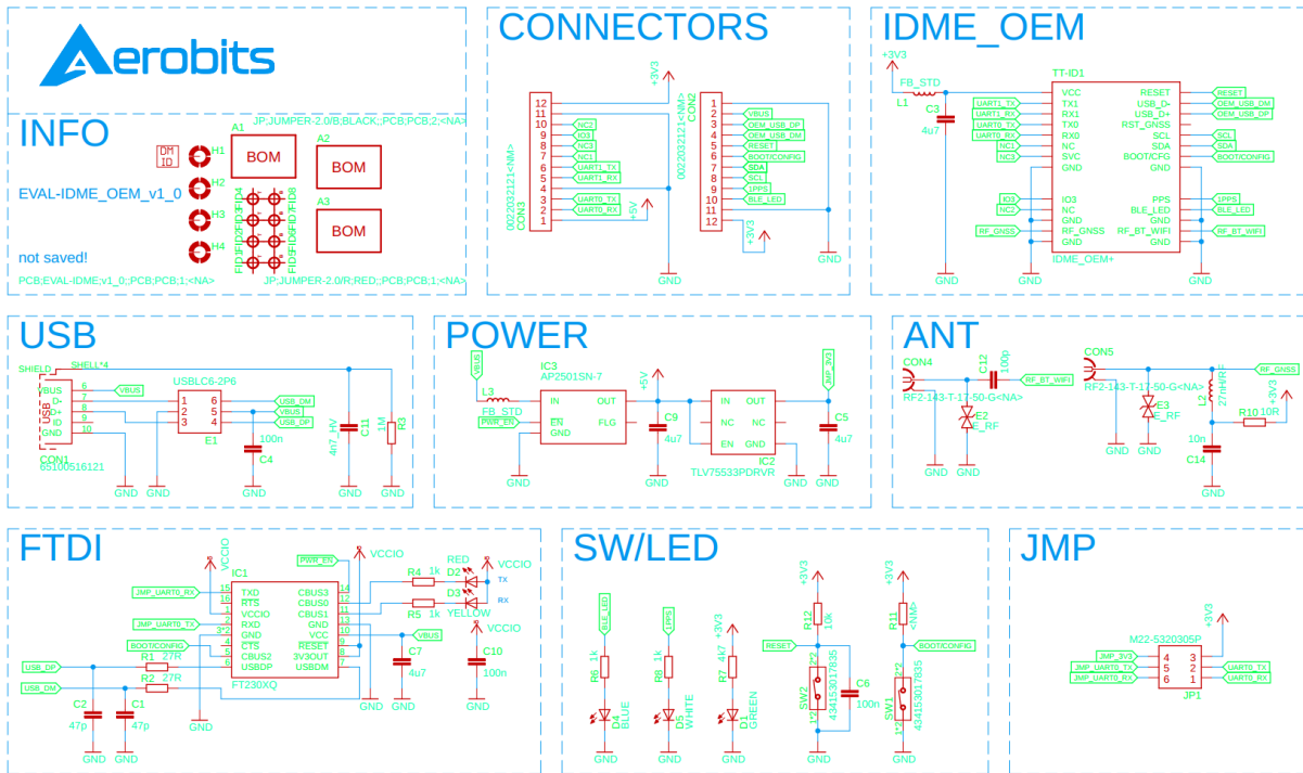
Figure 4: Electrical diagram of EVAL TT-RW1
