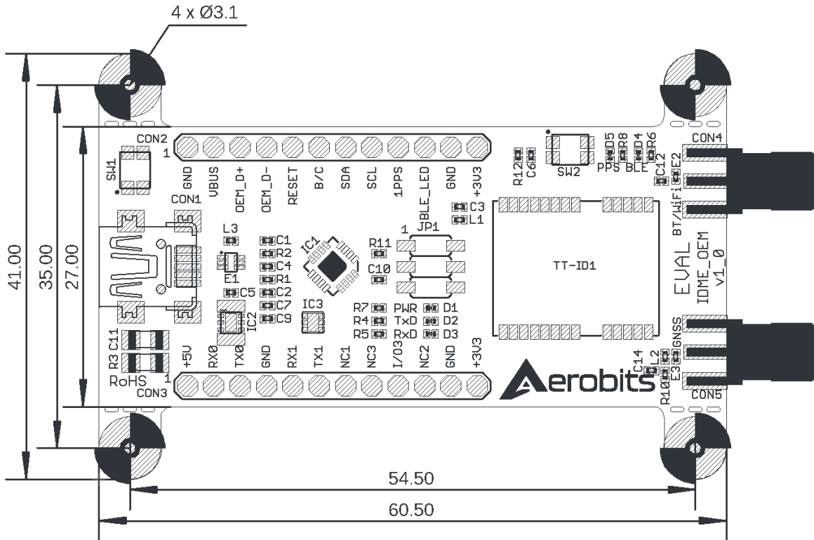
Figure 5: Dimensions of EVAL TT-RW1
