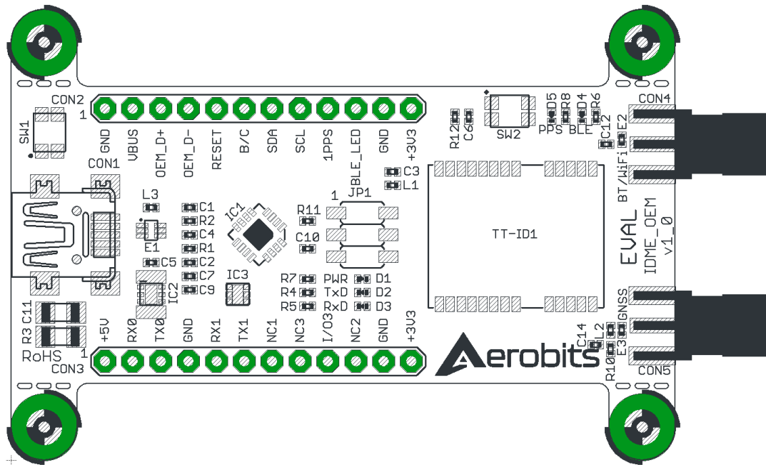
Figure 1: Top view of EVAL TT-RG1.
